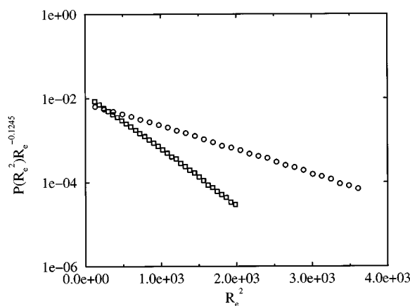
FIG. 9. The measured function p(R_e^2)R_e^{-0.1245} . Fits shows that \nu > 0.5 implying that the chains are slightly swollen at criticality.
