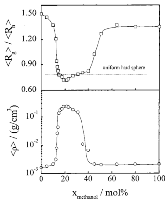
Figure 5. Methanol molar fraction ( x_{\text{methanol}} ) dependence of \langle R_g \rangle / \langle R_h \rangle and average chain density ( \rho ) of PNIPAM chains in methanol/water mixtures.
