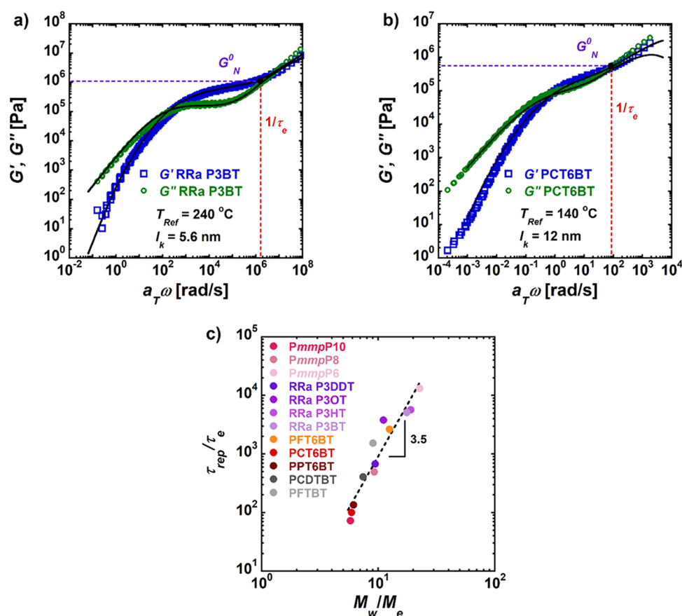
Figure 3. Master-curves of (a) RRa P3BT and (b) PCT6BT. Master-curves were generated using tTs and were horizontally shifted to reference temperatures of 240 and 140 ^{\circ}\text{C} , respectively, using shift factors a_T as shown in SI 6–9. The open symbols are experimental data, and the solid black curves are the fits to G' and G'' , generated from the BoB tube model, inputting the molecular mass distribution from GPC and assuming all chains are linear. The master-curves for the other 10 polymers tested can be seen in SI 3–5. (c) Ratio of the reptation time, \tau_{rep} , and Rouse time of an entanglement strand, \tau_e , as a function of the number of entanglements along the chain for all 12 conjugated polymers.
